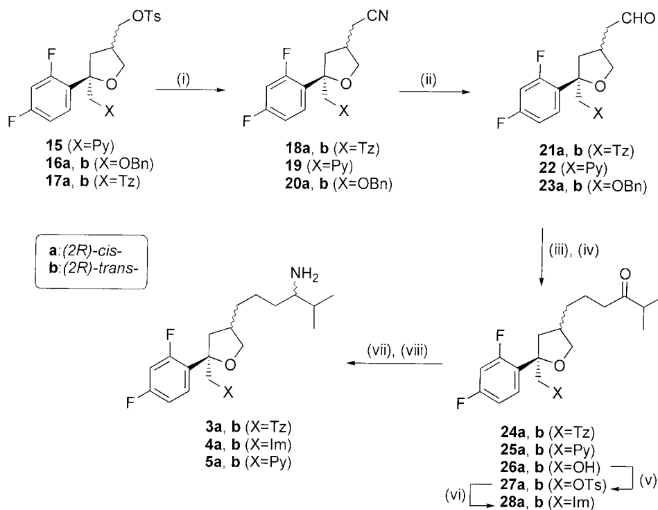
Scheme 2. (i) KCN, DMSO, 50–55 °C; (ii) DIBAL, toluene; (iii) dimethyl 3-methyl-2-oxobutylphosphonate, DBU, LiCl, MeCN, rt; (iv) H_2 , Pd-C, EtOH, rt; (v) TsCl, TEA, DMAP, CH_2Cl_2 , rt; (vi) Na-imidazole, DMPU, 100 °C; (vii) NH_2OHHCl , pyridine, EtOH, rt; (viii) NaBH_4 , NiCl_2 \cdot 6H_2O , MeOH.
