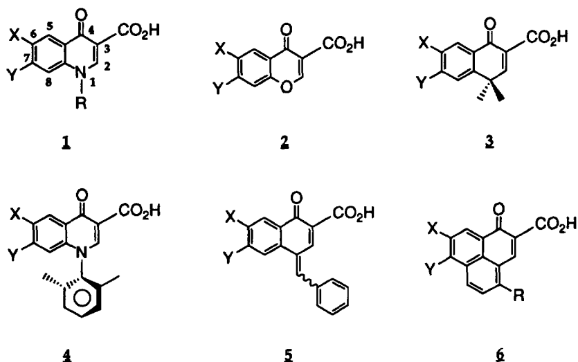
Figure 1. Quinolone and Geometric Analogues
